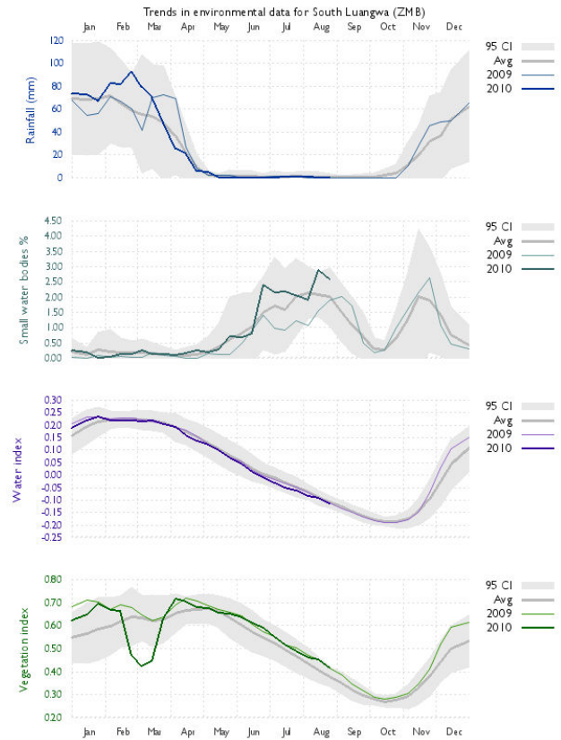
Figure 2: Dekadal behaviour (situation on 20/08/2010) of environmental factors (rainfall, small water bodies, vegetation indices: NDWI, NDVI) observed in the South Luangwa NP (Zambia) plotted against the averaged data of the previous year and longer term trends. Dark gray lines are the average for each dekad based on the available time series. Light grey areas indicate the 95% confidence limits around these averages.
